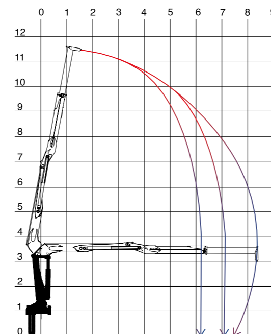
Principle sketch of how lifting force is affected by the extension.
